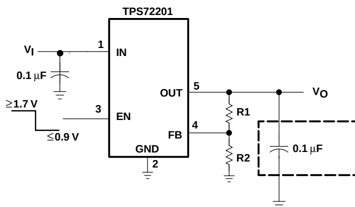
Figure 18. TPS72201 Adjustable LDO Regulator Programming
