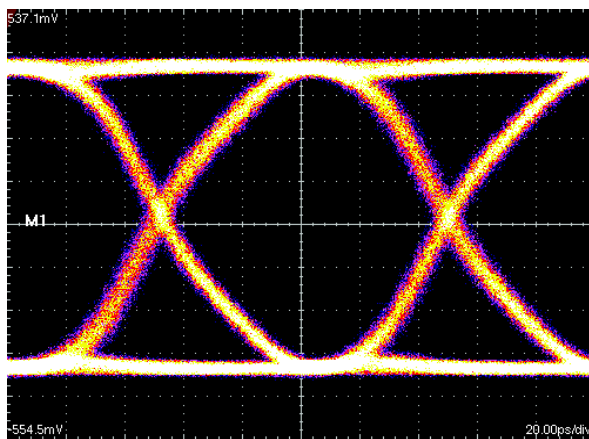
10 Gbps Eye Diagram With ESD8704
