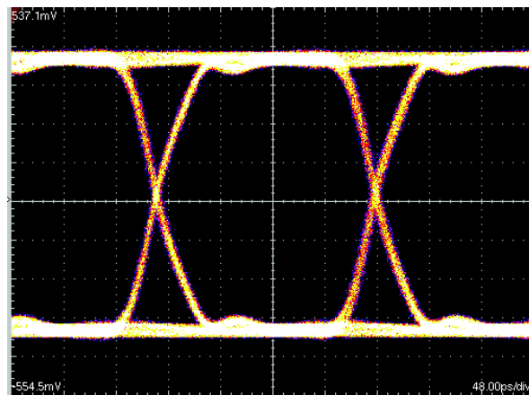
5 Gbps Eye Diagram With ESD8704
