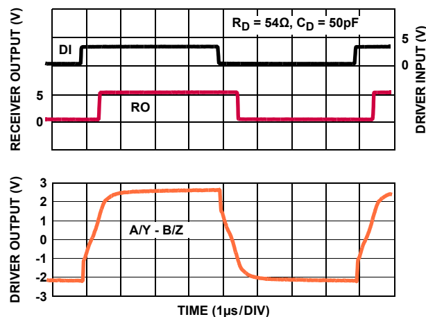
FIGURE 26. DRIVER AND RECEIVER WAVEFORMS (ISL32490E, ISL32492E)
