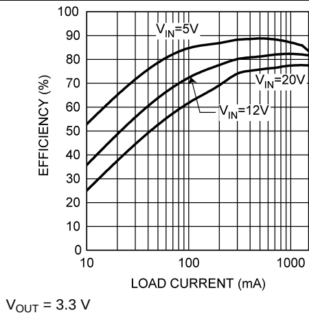
Figure 3. Efficiency vs Load Current – X Version
