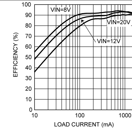
Figure 2. Efficiency vs Load Current – Y Version
