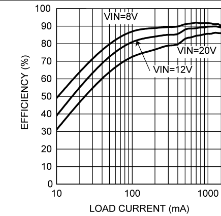
Figure 1. Efficiency vs Load Current – X Version
