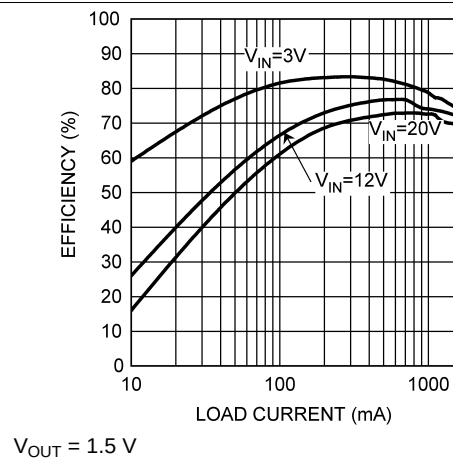
Figure 6. Efficiency vs Load Current – Y Version
