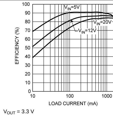
Figure 4. Efficiency vs Load Current – Y Version
