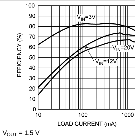
Figure 5. Efficiency vs Load Current – X Version
