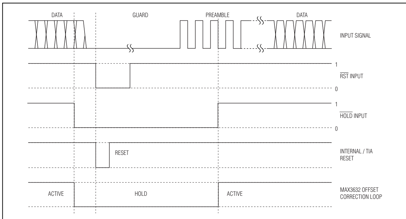
Figure 10. \overline{\text{RST}} / \overline{\text{HOLD}} Timing Method 3
