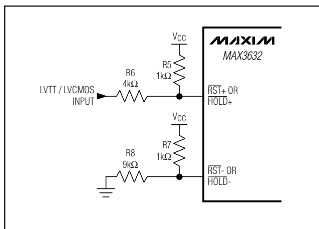
Figure 12. Interfacing \overline{\text{RST}} or \text{HOLD} to Single-Ended LVTTTL/LVCMOS
