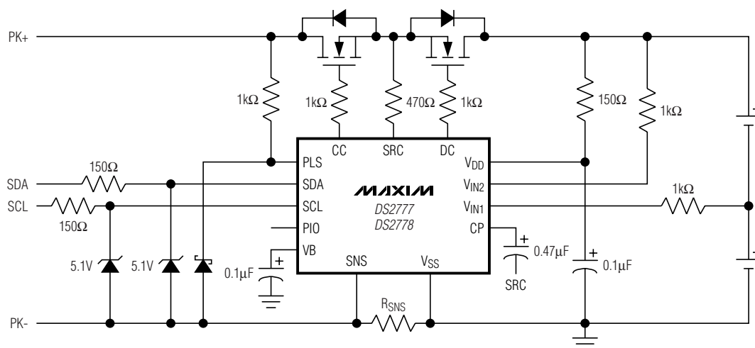
DS2777/DS2778 Typical Application Circuit
