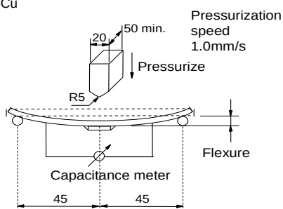
Fig.1 (in mm)
