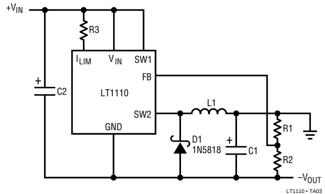
Figure 7. Positive-to-Negative Converter
