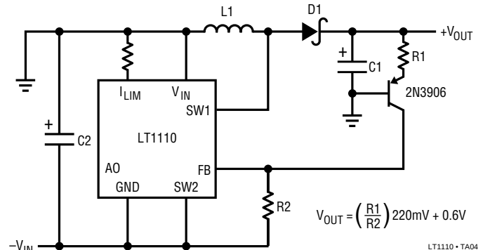
Figure 8. Negative-to-Positive Converter
