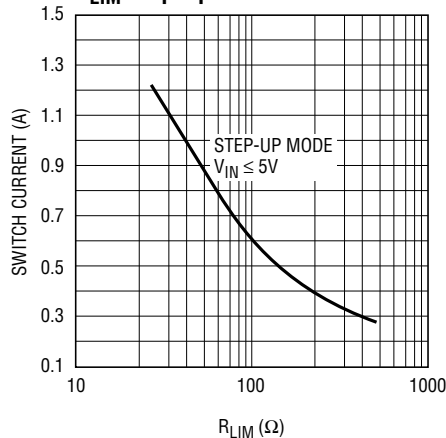
Maximum Switch Current vs RLIM Step-Up
