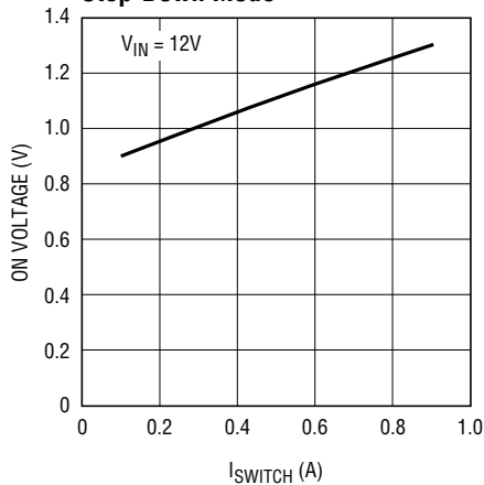
Switch On Voltage Step-Down Mode
