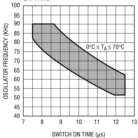
Minimum/Maximum Frequency vs On Time
