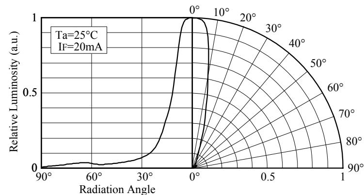
■ Directivity (NSPW300BS)
