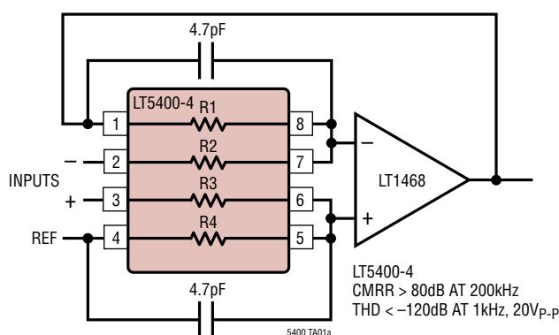
Difference Amplifier
