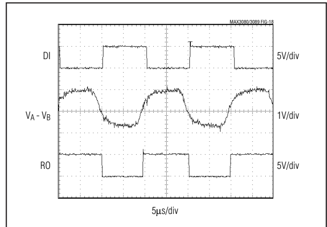
Figure 19. MAX3080E/MAX3081E/MAX3082E, and MAX3089E with \text{SRL} = Unconnected, System Differential Voltage at 50kHz Driving 4000ft of Cable
