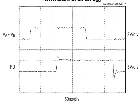
RECEIVER PROPAGATION DELAY MAX3080E-MAX3085E AND MAX3089E WITH SRL = OPEN OR V_{CC}
