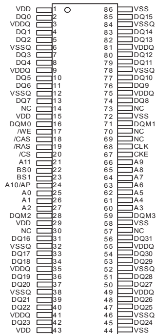
Pin Assignment (Top View)
