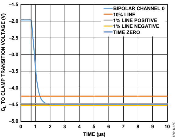
Figure 34. Closed Loop to Clamp Settling Time
