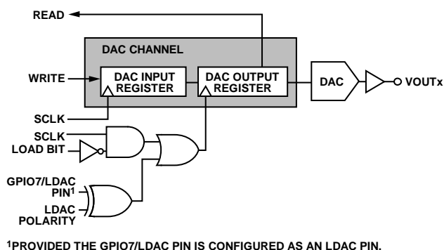
Figure 48. Simplified Diagram of Input Loading Circuitry for a Single DAC
