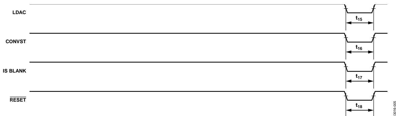
Figure 5. Asynchronous Inputs
