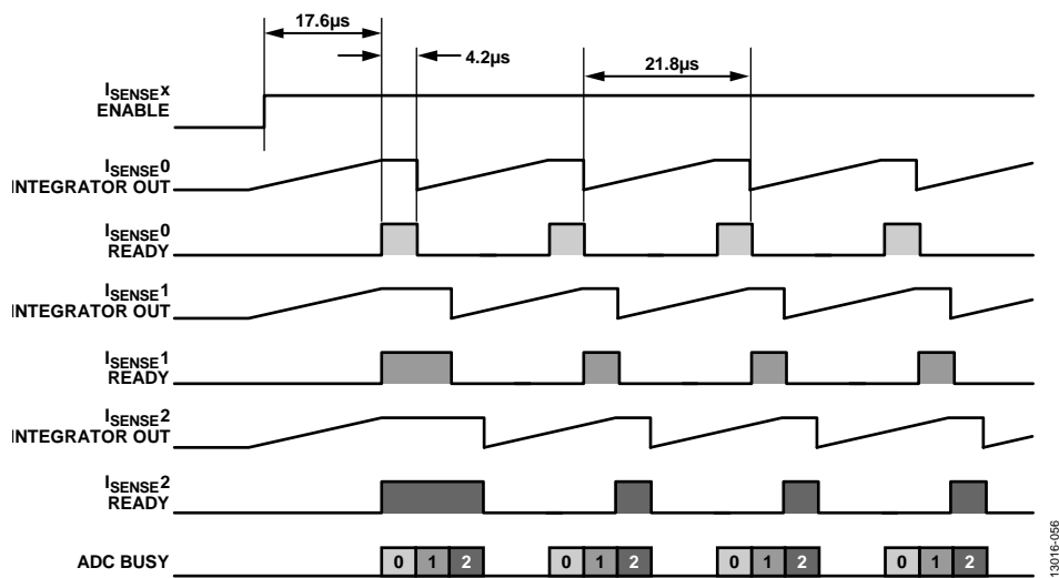
Figure 57. Conversion and Integration Internal Timing Example 1
