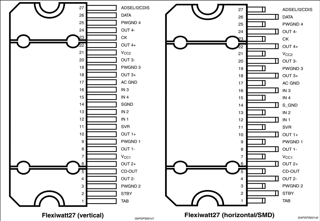
Figure 5. Pin connection diagram of the Flexiwatt27 (top of view)
