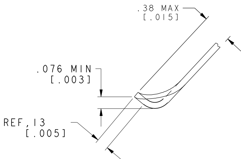
TIP DETAIL
