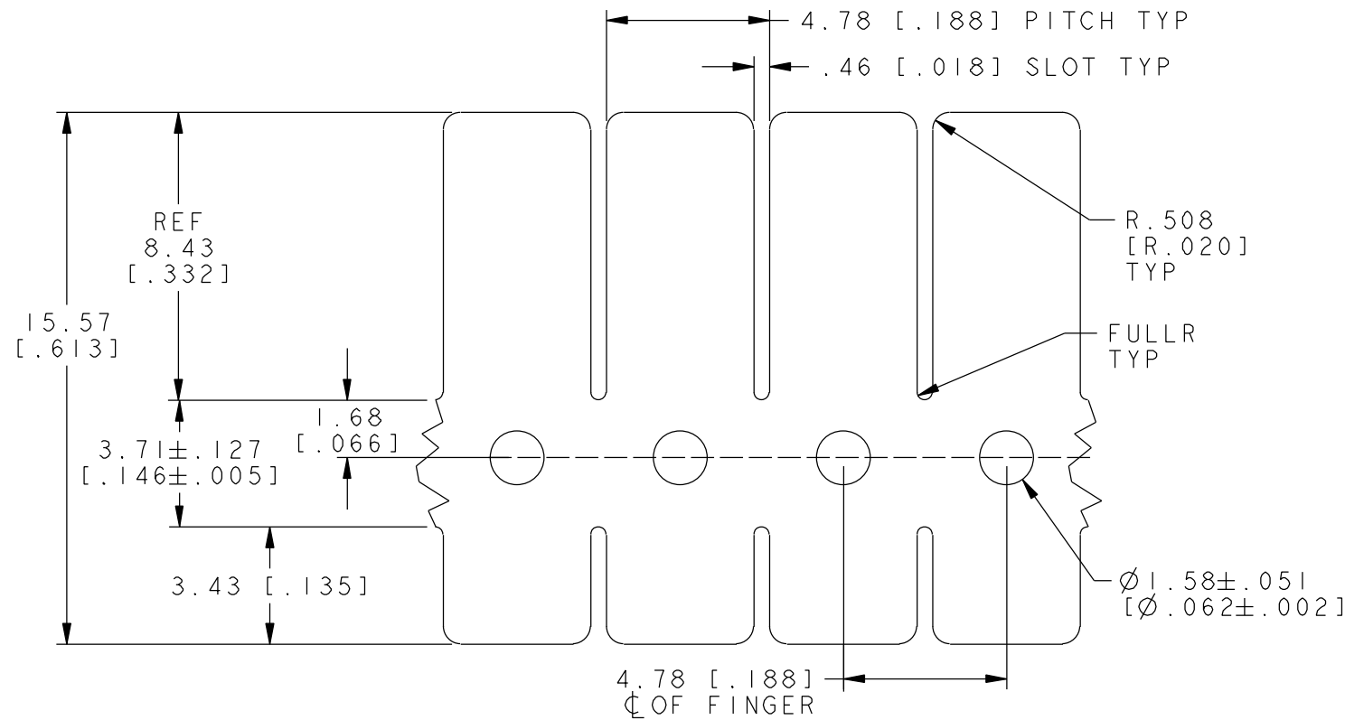
FLAT PATTERN
