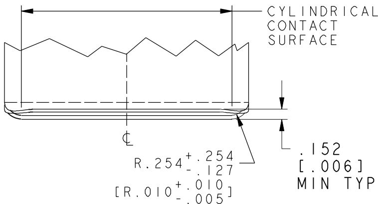
FINGER DETAIL
