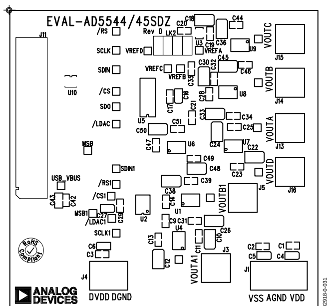
Figure 30. Silkscreen
