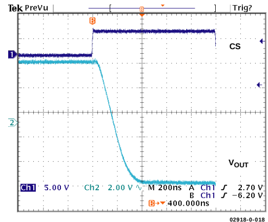
Figure 15. Settling Time
