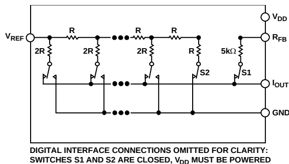
Figure 17. Equivalent R-2R DAC Circuit
