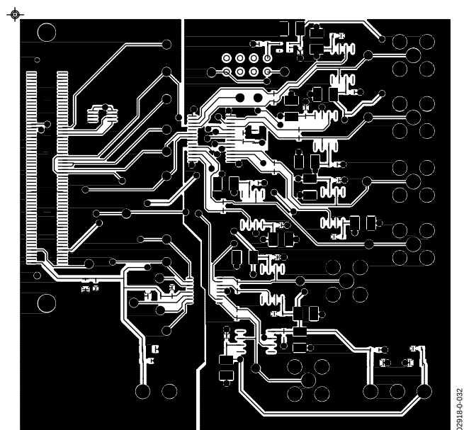
Figure 31. Component Side
