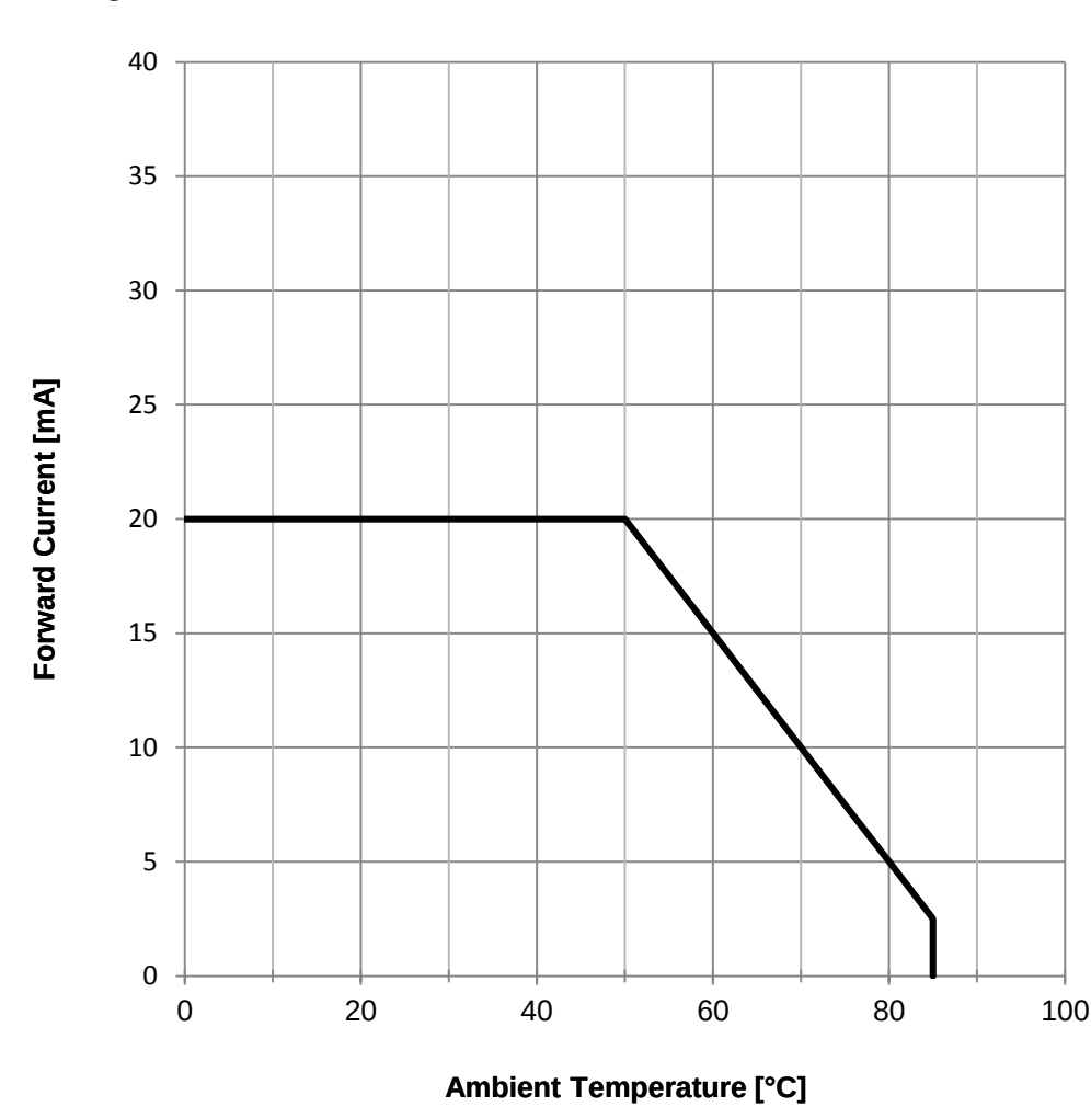
Derating Curve:
