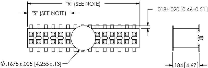
FIG 6 -K: OPTION (POLYIMIDE FILM PAD) (DIFFERENT AS SHOWN, OTHERWISE SAME AS FIG 1)
