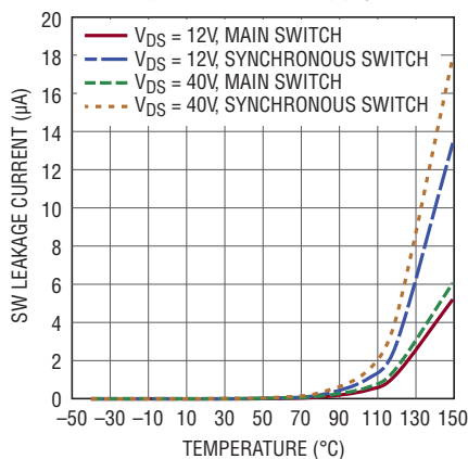
Switch Pin Leakage vs Temperature and Supply
