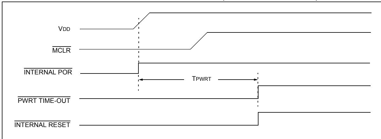
FIGURE 5-4: TIME-OUT SEQUENCE ON POWER-UP ( \overline{\text{MCLR}} NOT TIED TO \text{V}_{\text{DD}} ): CASE 1
