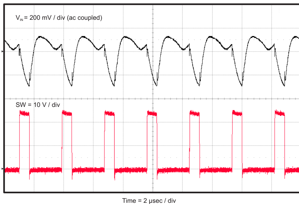
Figure 10. TPS54335EVM-556 Input Ripple
