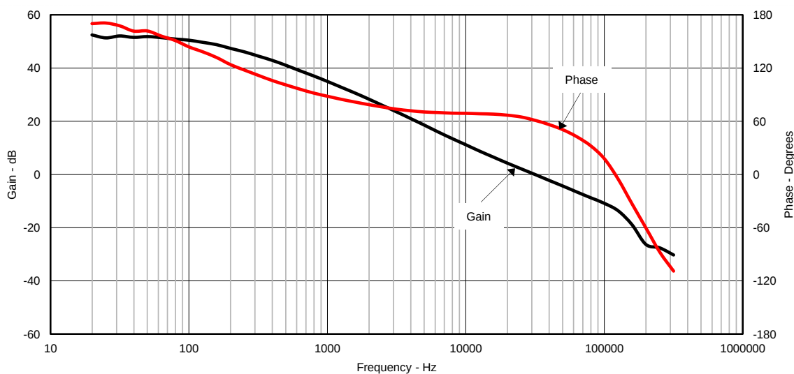
Figure 6. TPS54335EVM-556 Loop Response
