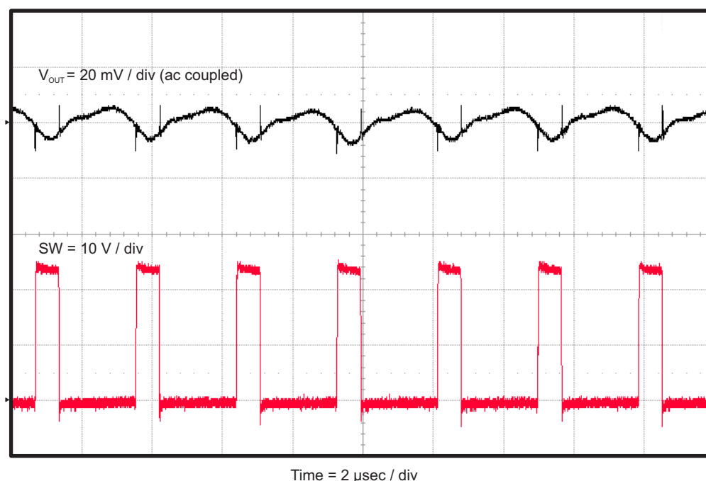
Figure 7. TPS54335EVM-556 Output Ripple, I_{OUT} = 3 A
