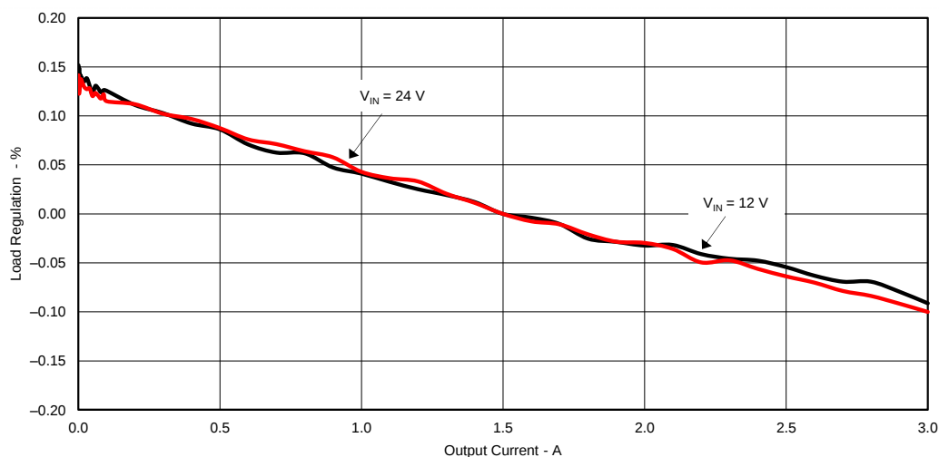
Figure 3. TPS54335EVM-556 Load Regulation
