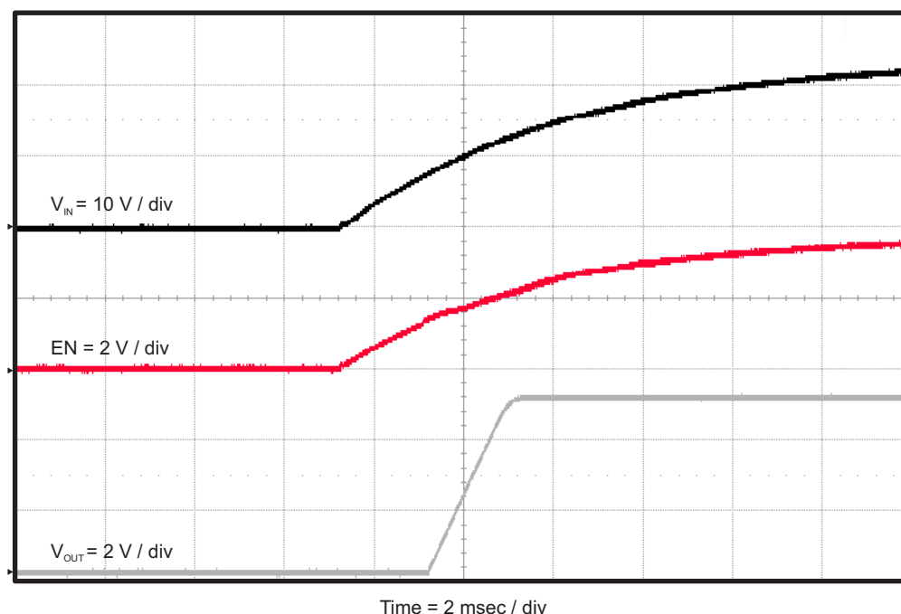
Figure 11. TPS54335EVM-556 Start-Up Relative to V_{IN}
