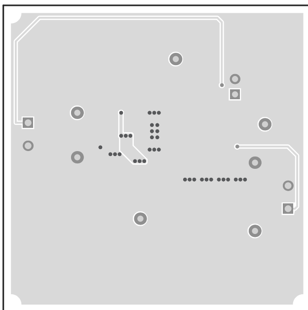
Figure 17. TPS54335EVM-556 Bottom-Side Layout
