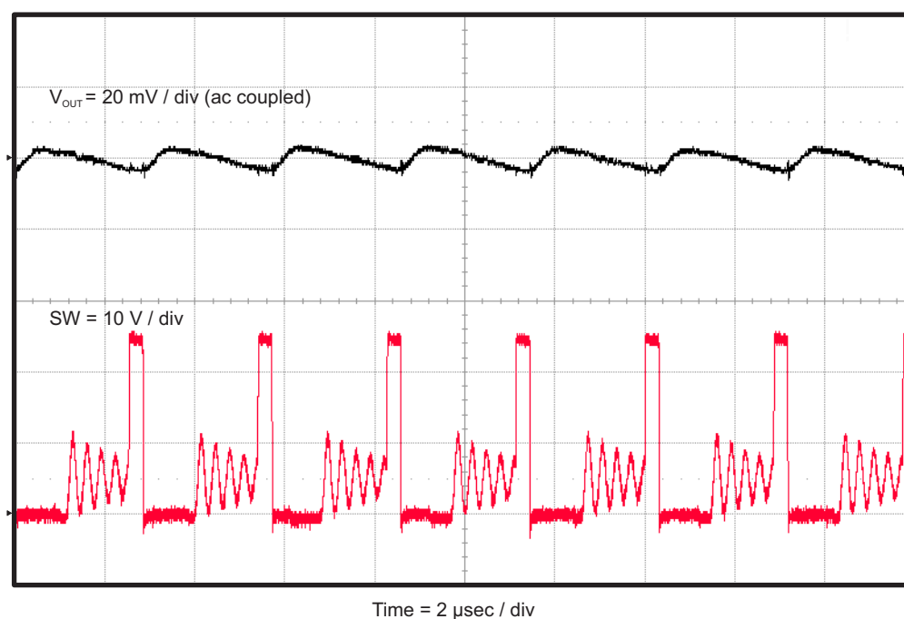
Figure 8. TPS54335EVM-556 Output Ripple, I_{OUT} = 100 mA
