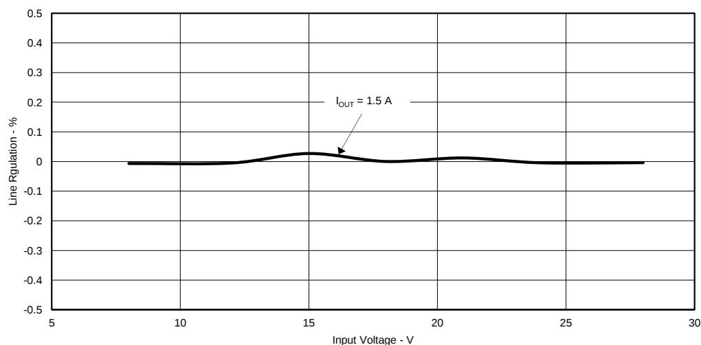
Figure 4. TPS54335EVM-556 Line Regulation
