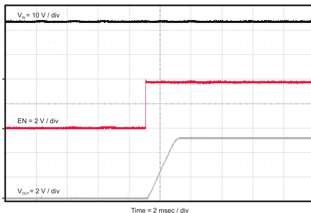
Figure 12. TPS54335EVM-556 Start-up Relative to Enable
