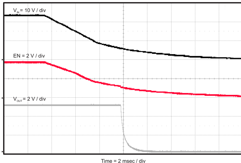
Figure 13. TPS54335EVM-556 Shut-down Relative to V_{IN}
