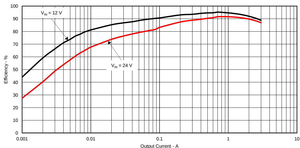
Figure 2. TPS54335EVM-556 Low Current Efficiency
