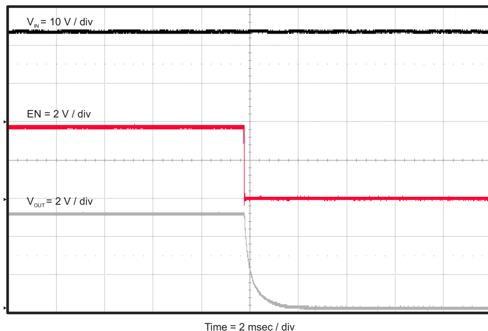
Figure 14. TPS54335EVM-556 Shut-down Relative to EN
