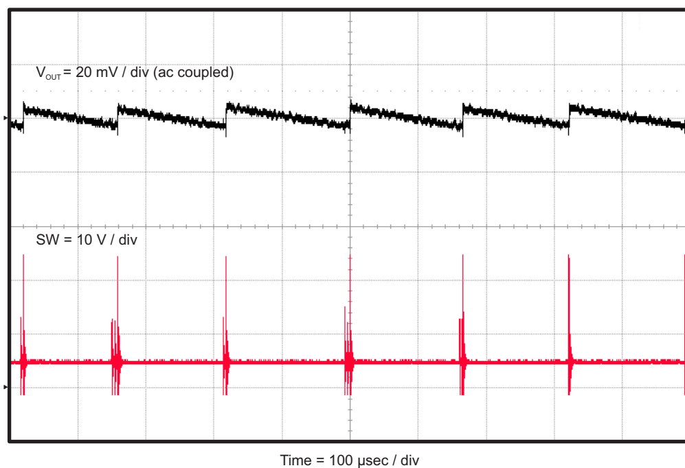
Figure 9. TPS54335EVM-556 Output Ripple, I_{OUT} = 0 A
