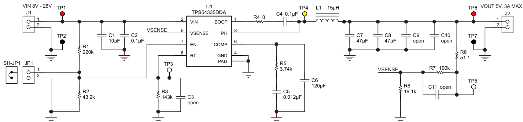
Figure 18. TPS54335EVM-556 Schematic
