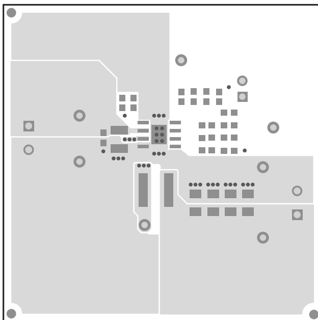
Figure 16. TPS54335EVM-556 Top-Side Layout 3
