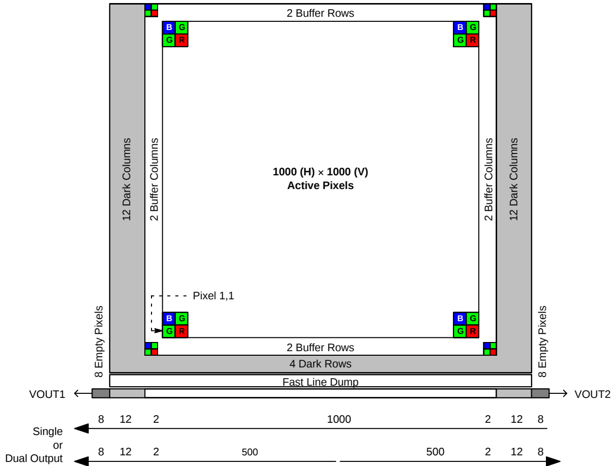
Figure 2. Block Diagram
