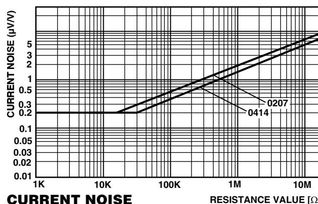
CURRENT NOISE
