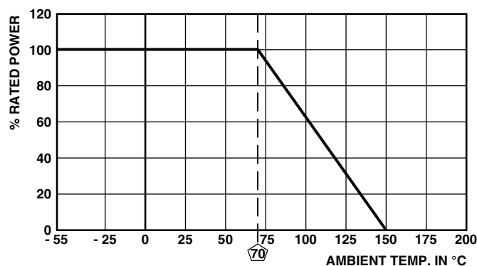
DERATING
