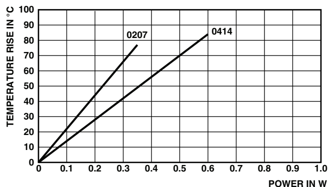
TEMPERATURE RISE
