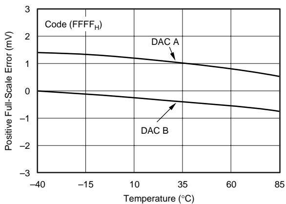
POSITIVE FULL-SCALE ERROR vs TEMPERATURE
