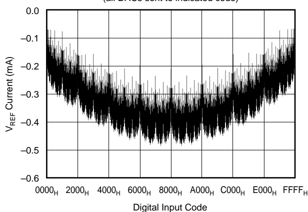
V_{REFL} CURRENT vs CODE (all DACs sent to indicated code)
