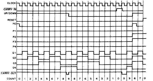
Fig. 15 — Timing Diagram for CD4510B.
