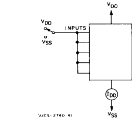
Fig. 11 - Quiescent-device-current test circuit.
