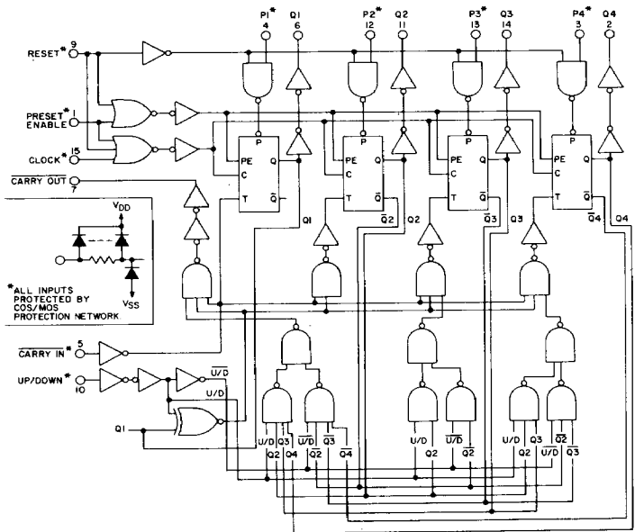
Fig.10 - Logic Diagram for CD4516B.
