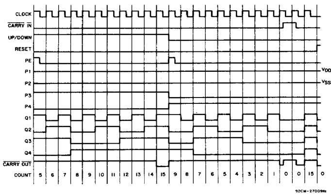
Fig. 16 — Timing diagram for CD4516B.
