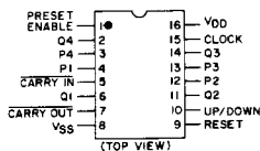
CD4510B, CD4516B TERMINAL ASSIGNMENT
