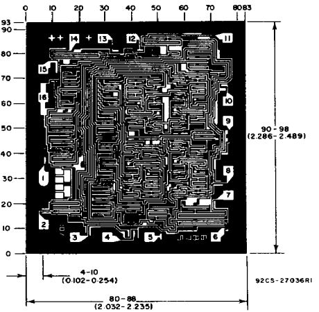
Dimensions and Pad Layout for CD4516BH.
