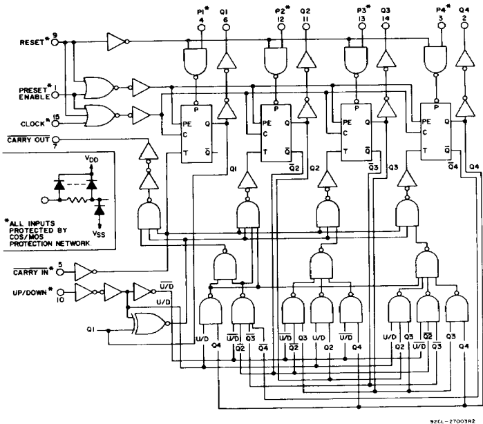
Fig.3 — Logic Diagram for CD4510B.
