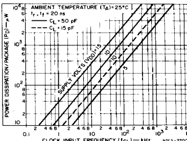
Fig.9 - Typical dynamic power dissipation vs. frequency.
