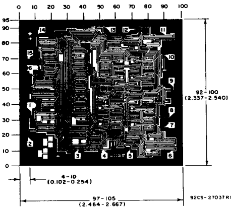
Dimensions and Pad Layout for CD4510BH.
