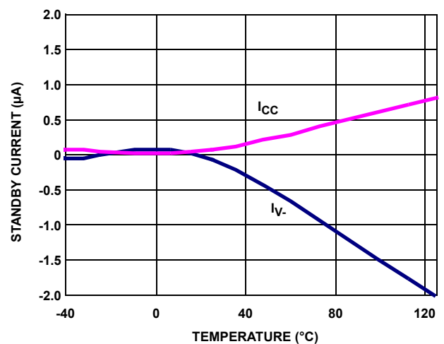
FIGURE 2. STANDBY I_{CC} and I_{q-} vs TEMPERATURE
