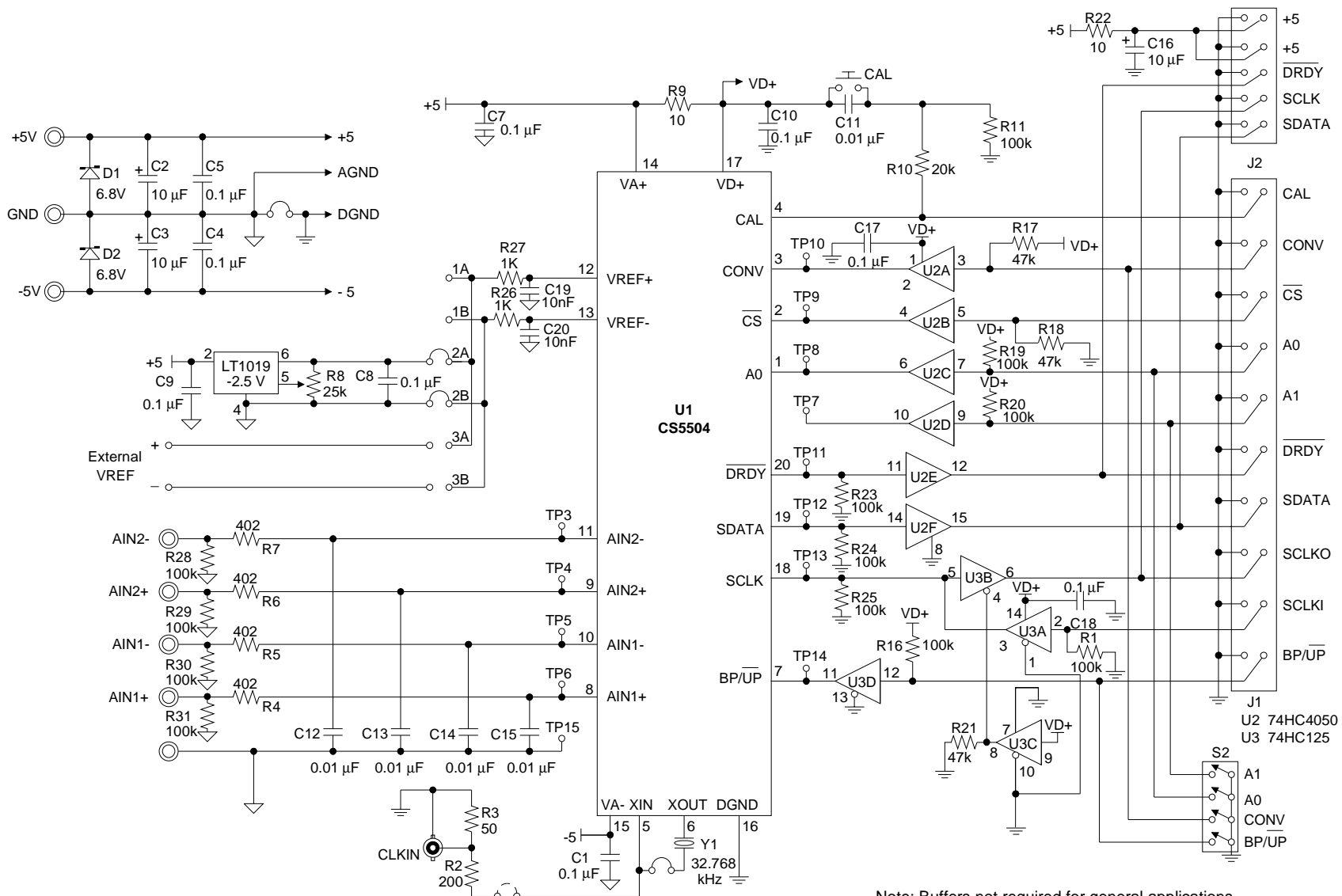
Figure 1. ADC Connections
