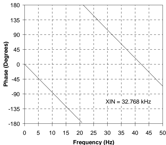
Figure 7. Filter Phase Plot to 50 Hz
