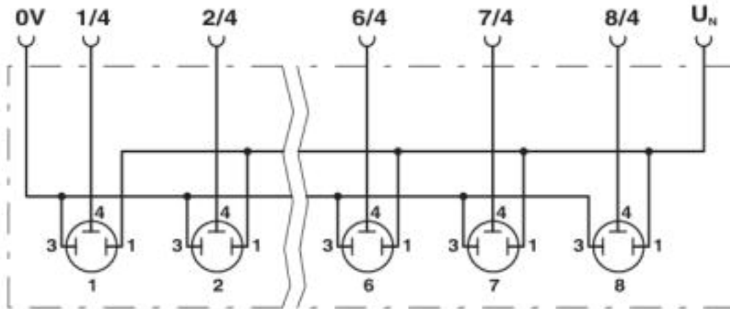
Schematic diagram
