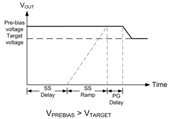
Figure 20. Output Responses to Pre-bias Voltages
