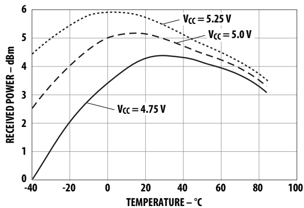
Figure 7. Typical POF receiver overdrive P_{RL,max} at 10 MBd vs. temperature and power supply voltage
