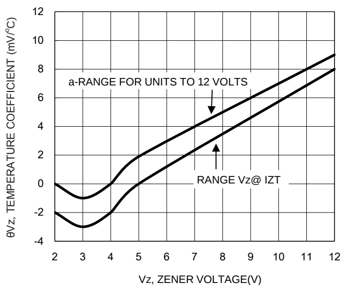
Fig7. Temperature Coefficients
