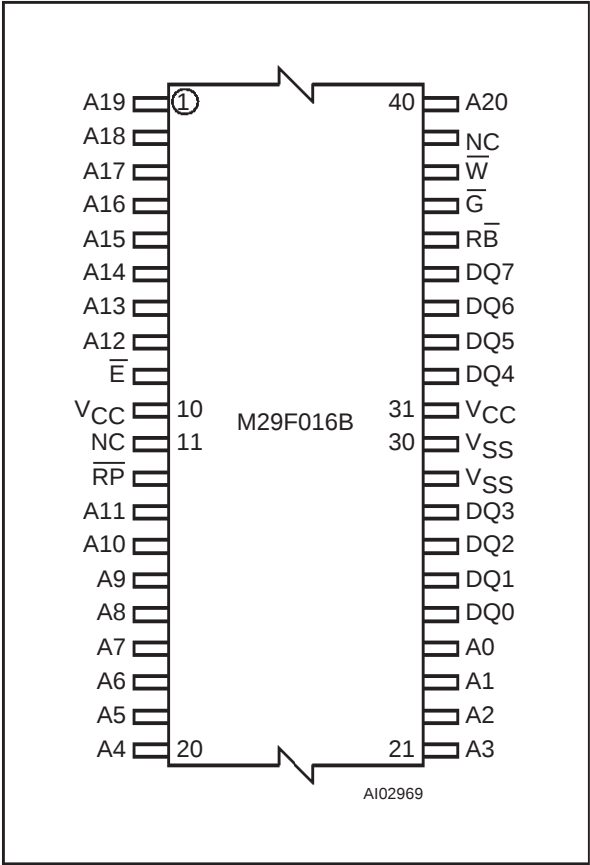
Figure 2. TSOP Connections
