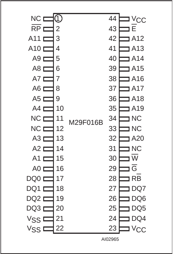
Figure 3. SO Connections
