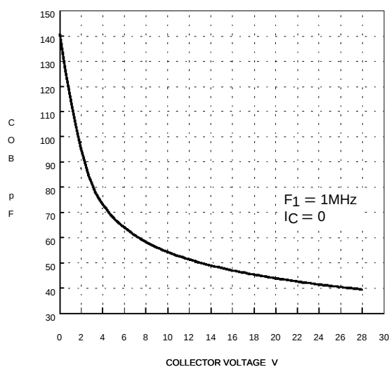
OUTPUT CAPACITANCE vs C-B VOLTAGE
