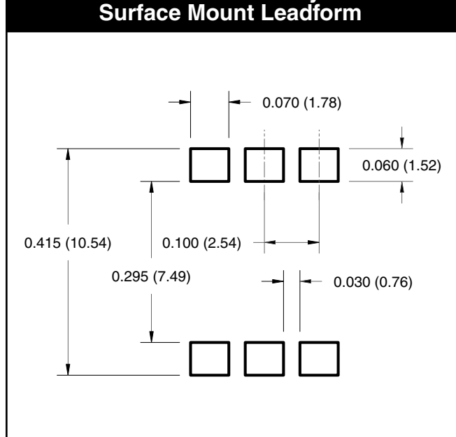
Recommended Pad Layout for Surface Mount Leadform
