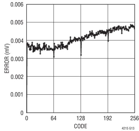
Total Unadjusted Error vs Code (ADIN)
