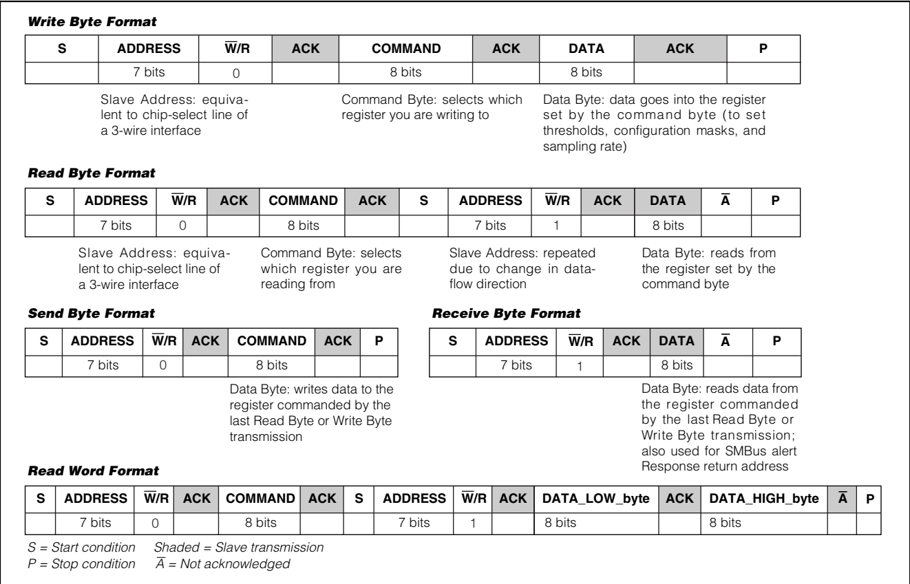
Figure 2. SMBus Protocols
