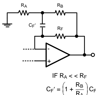
Figure 59. Obtaining Small C_F from large C_F'
