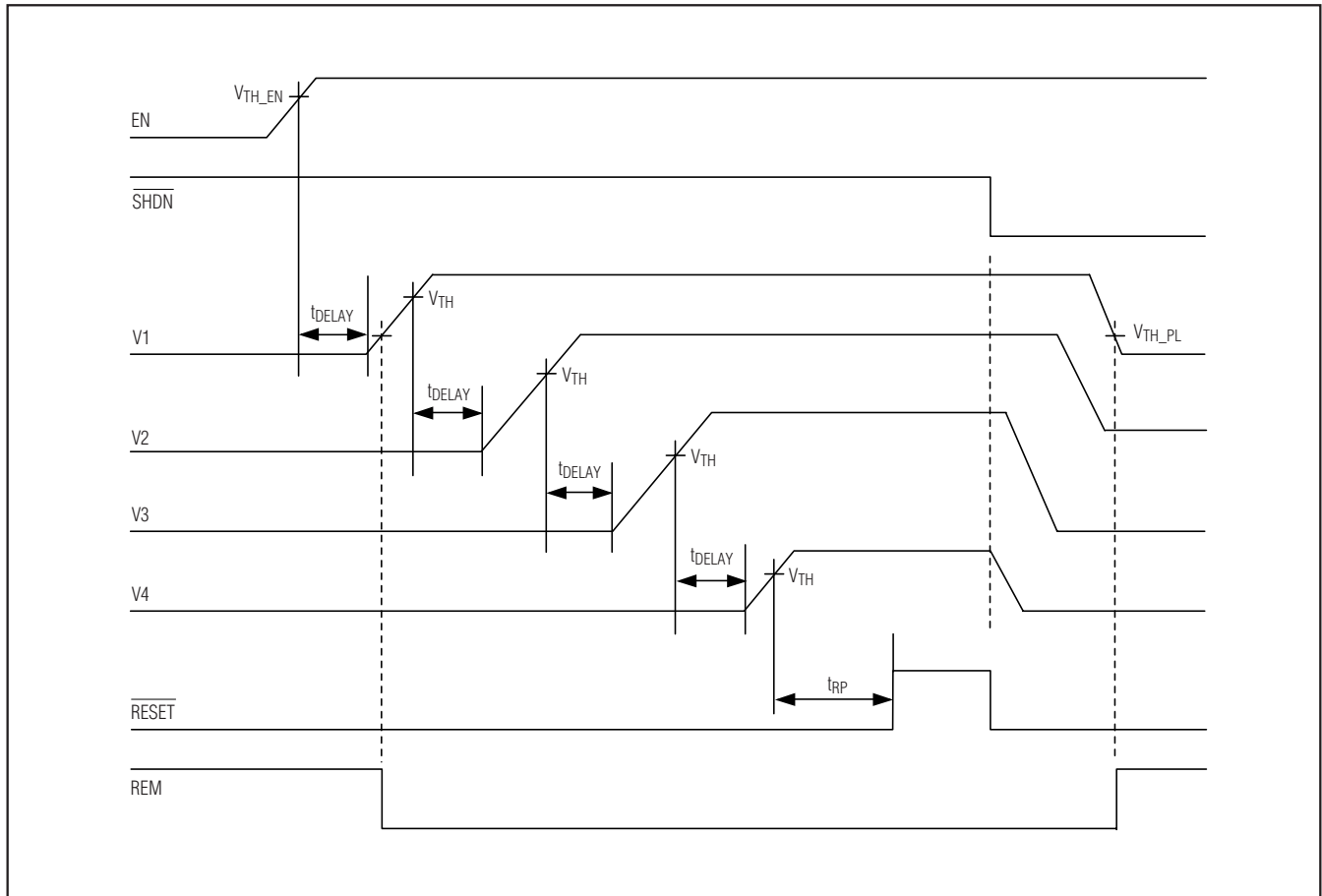
Figure 1. Sequencing Timing Diagram with Reverse Order Power-Down Using \overline{\text{SHDN}}
