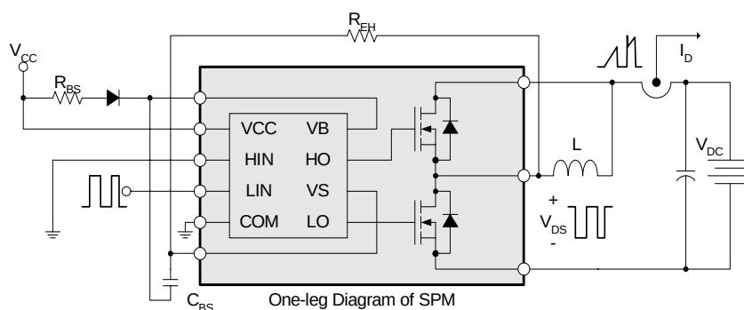
(b) Turn-off
