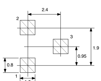
OUTLINE 33 RECOMMENDED P.C.B. LAYOUT
