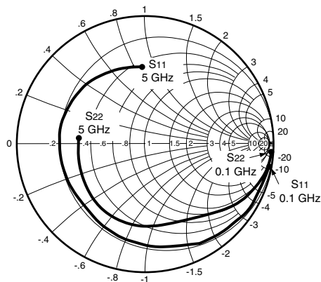
Coordinates in Ohms Frequency in GHz ( V_{CE} = 0.5\text{ V} , I_C = 0.5\text{ mA} )
