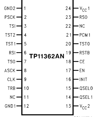
Top View Order Number TP11362AN See NS Package Number N24A
