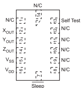
Figure 4. Pinout Description
