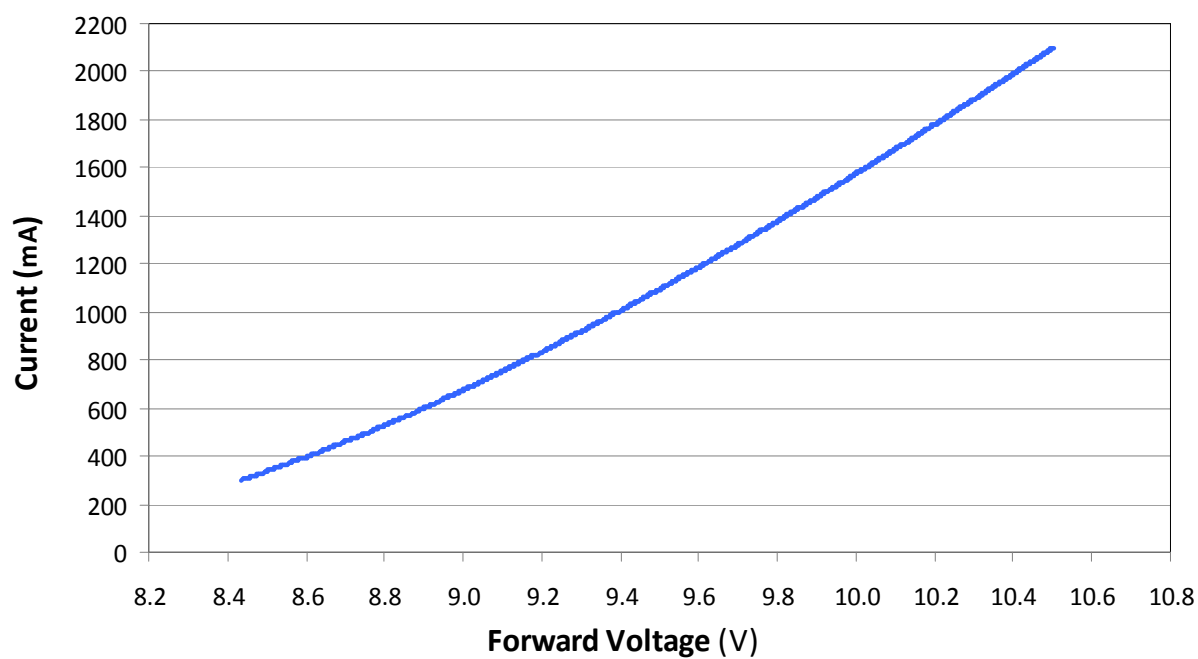
Figure 17: Typical Current vs. Voltage, BXRA-N0402
