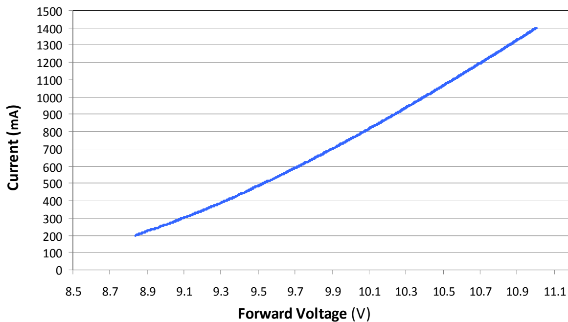
Figure 16: Typical Current vs. Voltage, BXRA-C0402
