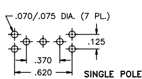
SINGLE POLE
