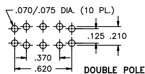
DOUBLE POLE
