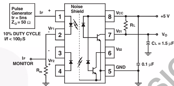
Test Circuit for HCPL-2530 and HCPL-2531
