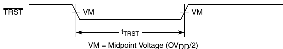
Figure 29. \overline{\text{TRST}} Timing Diagram
