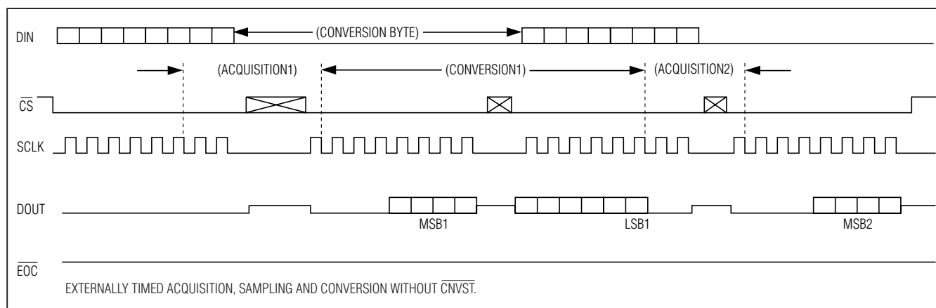
Figure 7. Clock Mode 11
