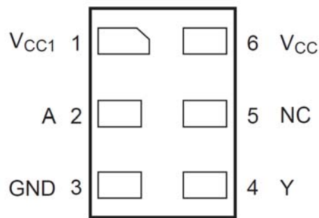
Figure 2. MicroPak™ (Top Through View)
