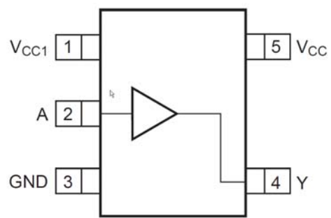
Figure 1. SC70 (Top View)
