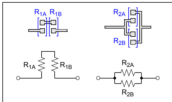
FIGURE 4-14: PCB Layout for Individual Resistors.
