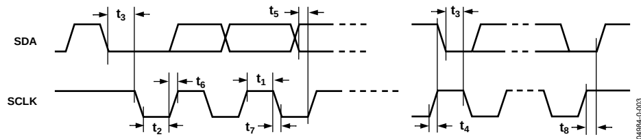
Figure 2. I²C Timing
