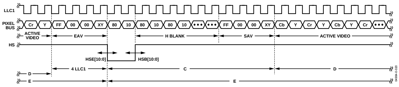
Figure 19. HS Timing
